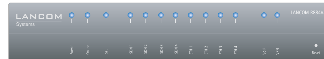
① Power ② Online ③ DSL ④ ISDN 1 ISDN 2 ISDN 3 ISDN 4 ⑤ ETH 1 ETH 2 ETH 3 ETH 4 ⑥ VoIP ⑦ VPN ⑧ Reset
